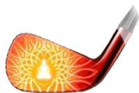
Nirvana 5 Accuracy: 97
