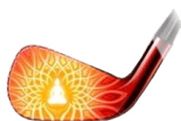
Nirvana 7 Accuracy: 100
