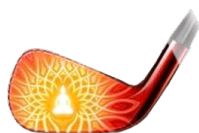
Nirvana 6 Accuracy: 97
